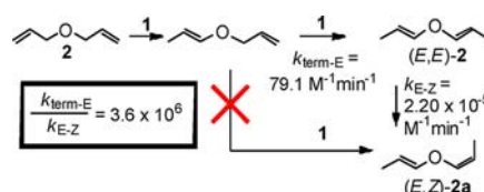
Scheme 1. Alkene Positional Isomerization Is Much Faster Than Geometrical Isomerization
