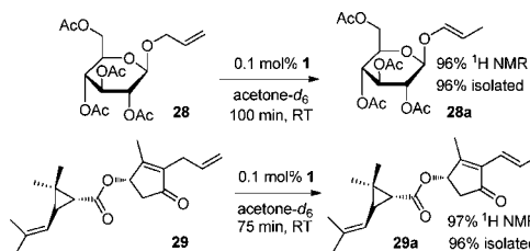
Scheme 2. Alkene Isomerization of Biologically Active Molecules at Low Catalytic Loading of 1
